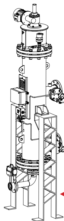
Vertical with lug support for skid mounting
